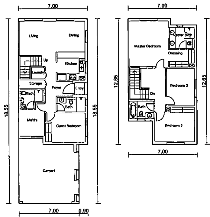
GROUND FLOOR PLAN VILLA NO: P1_122-21 FIRST FLOOR PLAN VILLA NO: P1_122-21
